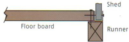
PEG FLOOR TO GROUND IN A WINDY AREA
